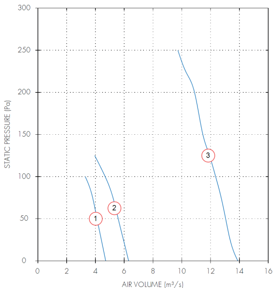
710 to 1000 dia. - 3 Phase - 6 Pole
