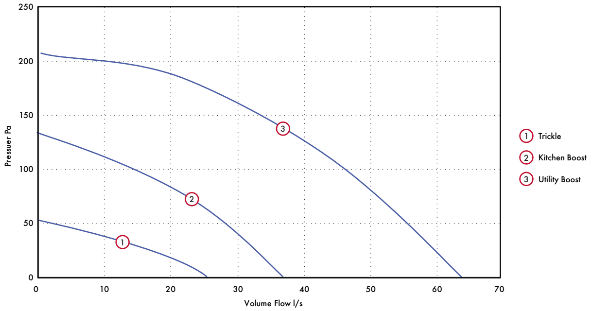
Performance @ 0 Pa
