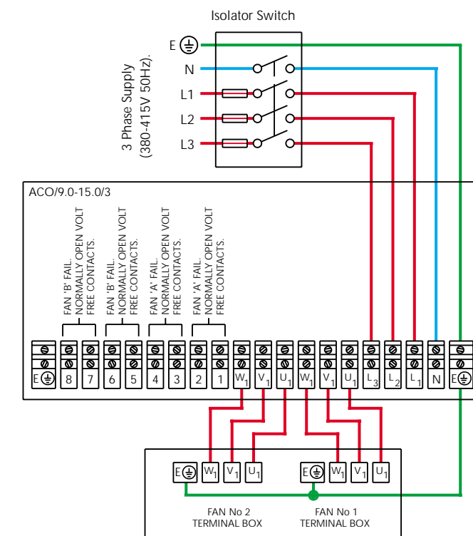
THREE PHASE FANS UP TO 4.0KW CONNECTED TO AN ACO/9.0-15.0/3 CONTROLLER
