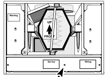
Remove bottom cover (3 screws)
