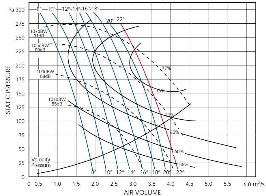
LC63A4 / 1ph
