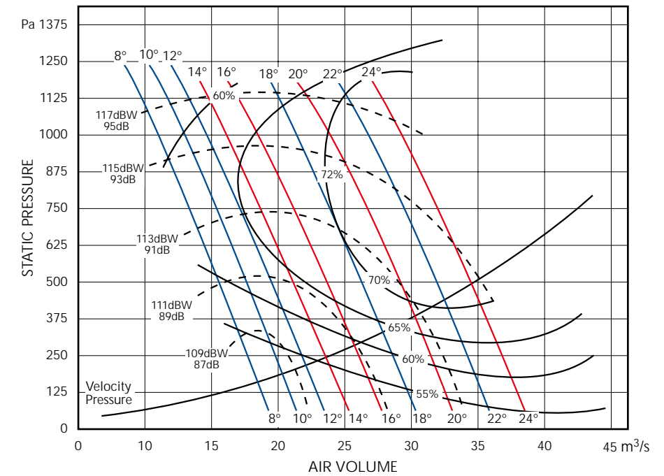
LC125A4 / 3ph
