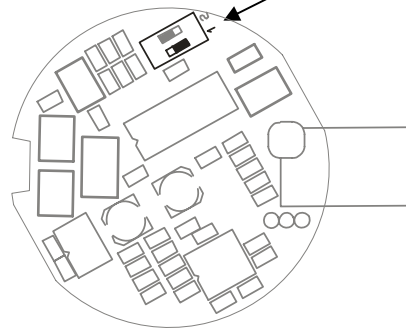
Fig.8. Constant flow option – using the flow sensor SW1 Dip switch
