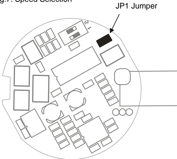
Fig.7. Speed Selection
