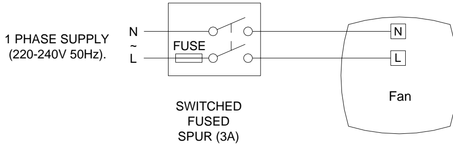
Fig.1 Continuous trickle (6l/s or 9l/s) with no boost facility
