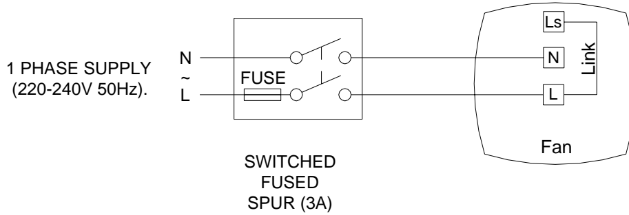
Fig.2 Continuous boost (15l/s) with no trickle facility
