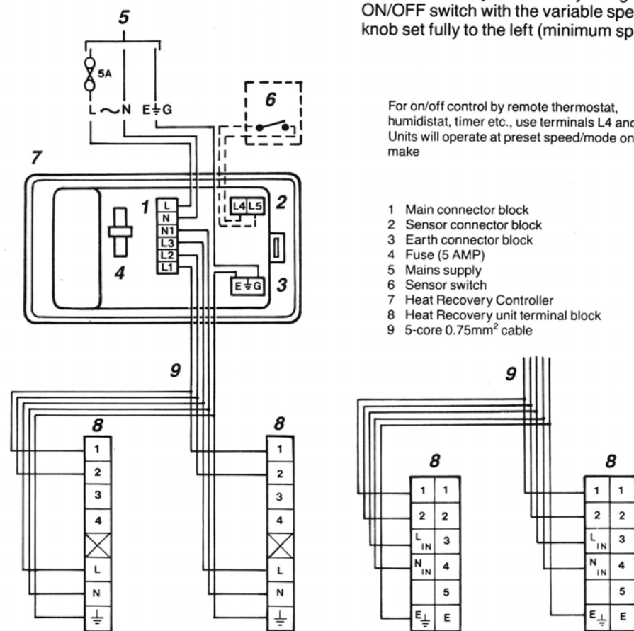
CURRENT HEAT RECOVERY VENTILATION UNIT TERMINAL BLOCKS AS FITTED TO HR500 MKIII AND HR500X (STOCK REFS 14101010B AND 14101070)
