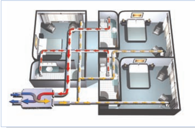
Typical network of hotel bathrooms/flats/apartments
